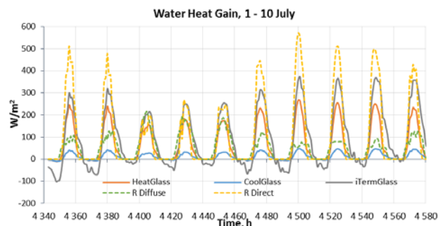
Fig.3. Water heat gain parameter as a function of total solar radiation for the first 10 days in July.
